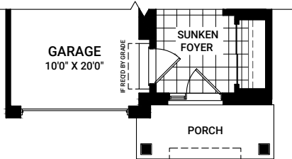
MAIN LEVEL ELEV. B
