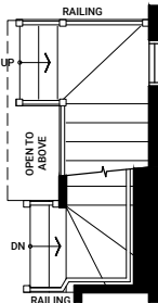
OPTIONAL STAIRS HALF WALL TO RAILING MAIN LEVEL
