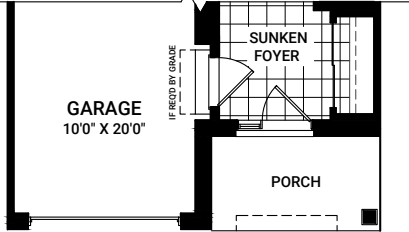
MAIN LEVEL ELEV. C
