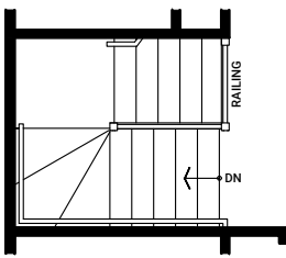
OPTIONAL STAIRS HALF WALL TO RAILING SECOND LEVEL
