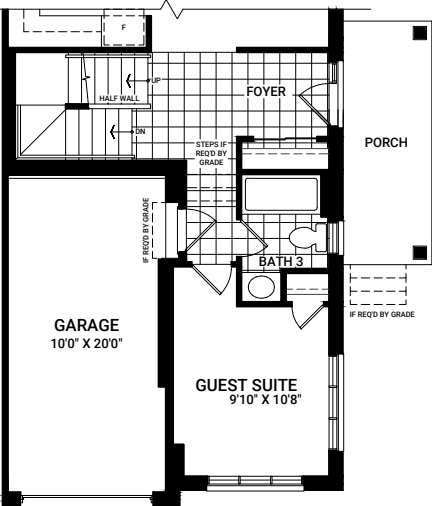
OPTIONAL MAIN FLOOR LAYOUT A
